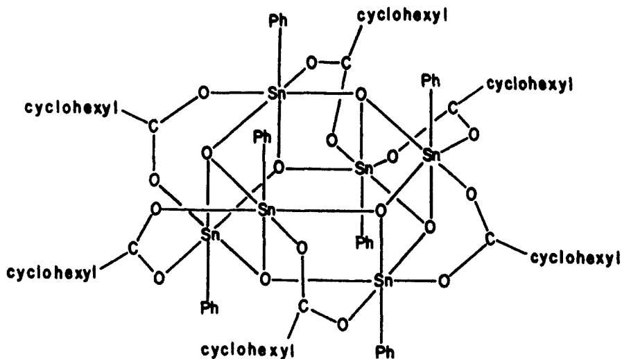
FIGURE 1 Hexagonal prismatic or "drum" structure of [\text{PhSn}(\text{O})\text{O}_2\text{CC}_6\text{H}_{11}]_6 . Reprinted with permission from ref 4. Copyright 1985 American Chemical Society.
