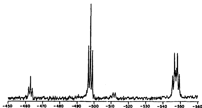
FIGURE 5 ^{119}\text{Sn} NMR spectrum ( \text{CDCl}_3 solution) of a reaction product of n -butylstannonic acid with dicyclohexylphosphinic acid in a 1:1.5 molar ratio, respectively. The three resonance patterns with increasing shielding are the cube [\text{n-BuSn}(\text{O})\text{O}_2\text{P}(\text{C}_6\text{H}_{11})_2]_4 at -462.8 ppm, the O-capped cluster [(\text{n-BuSn}(\text{OH})\text{O}_2\text{P}(\text{C}_6\text{H}_{11})_2)_3\text{O}][(\text{C}_6\text{H}_{11})_2\text{PO}_2] at -499.5 ppm, and the butterfly formulation [\text{n-BuSn}(\text{OH})(\text{O}_2\text{P}(\text{C}_6\text{H}_{11})_2)_2]_2 at -547.5 ppm. Reprinted with permission from ref 13. Copyright 1988 American Chemical Society.
