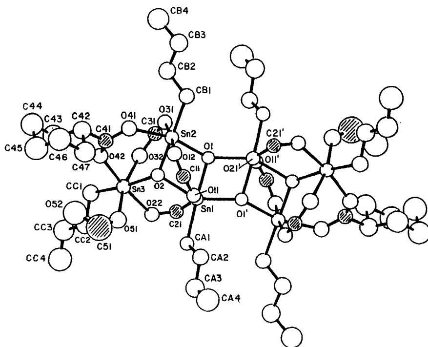
FIGURE 2 Ladder (open-drum) structure of [(n\text{-BuSn}(\text{O})\text{O}_2\text{CC}_6\text{H}_{11})_2n\text{-BuSn}(\text{O}_2\text{CC}_6\text{H}_{11})_3]_2 . Carbon atoms of only two of the cyclohexyl groups are shown. Reprinted with permission from ref 6. Copyright 1987 American Chemical Society.
