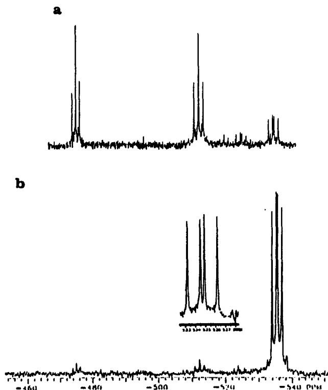
FIGURE 4 119 Sn NMR spectra of the crown cluster [(n\text{-BuSn}(\text{O})\text{O}_2\text{P}(\text{t-Bu})_2)(n\text{-BuSn}(\text{OH})\text{O}_2\text{P}(\text{t-Bu})_2)]_2[\text{H}][\text{O}_2\text{P}(\text{t-Bu})_2] , (a) from a recrystallization from a benzene-methylene chloride-ether mixture after reaction of a 1:2 molar ratio of n -BuSn(O)OH and ( t -Bu) 2 PO 2 H and (b) on the final product. The insert shows an enlarged spectrum of a pure sample. Reprinted with permission from ref 15. Copyright 1988 American Chemical Society.
