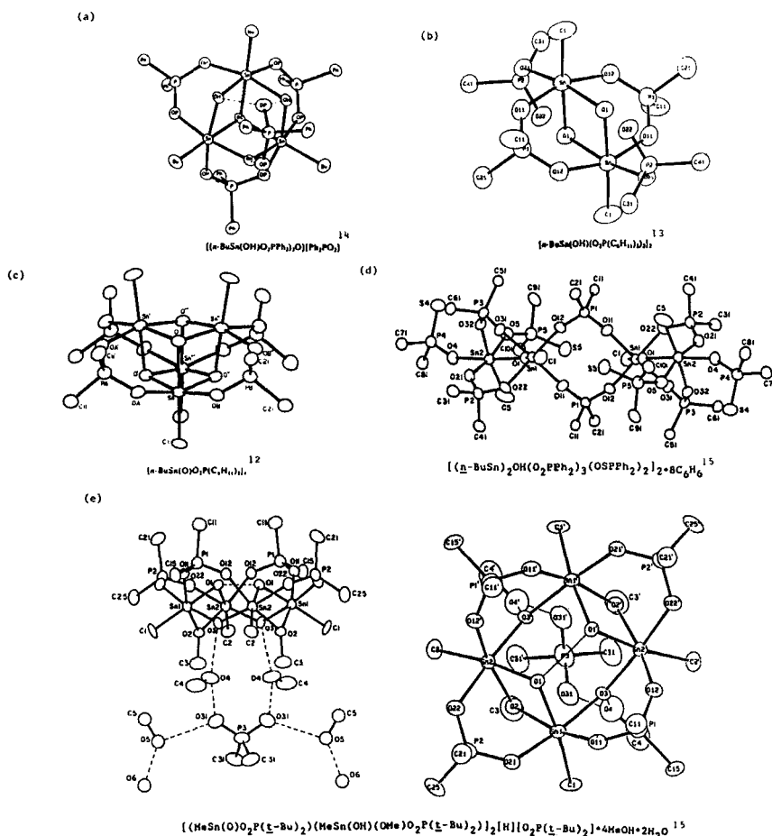
FIGURE 3 Examples of organotin clusters belong to the following structural types (references are indicated by superscripts): (a) an oxygen-capped cluster, (b) a butterfly formation, (c) a cube, (d) an extended form, and (e) a crown cluster (left view perpendicular to the crystallographic two-fold axis; right view looking down the two-fold axis). Pendant atoms and some solvent molecules have been removed for clarity. In addition, the hydrogen atoms attached to O1 and O1' have been deleted. Reprinted with permission from ref 12–15. Copyrights 1987 and 1988 American Chemical Society.
